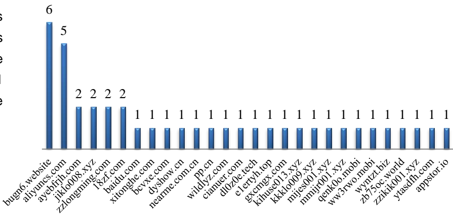
CNCERT Coordinated Platforms to Handle Mobile Malware (9/6-9/12)
